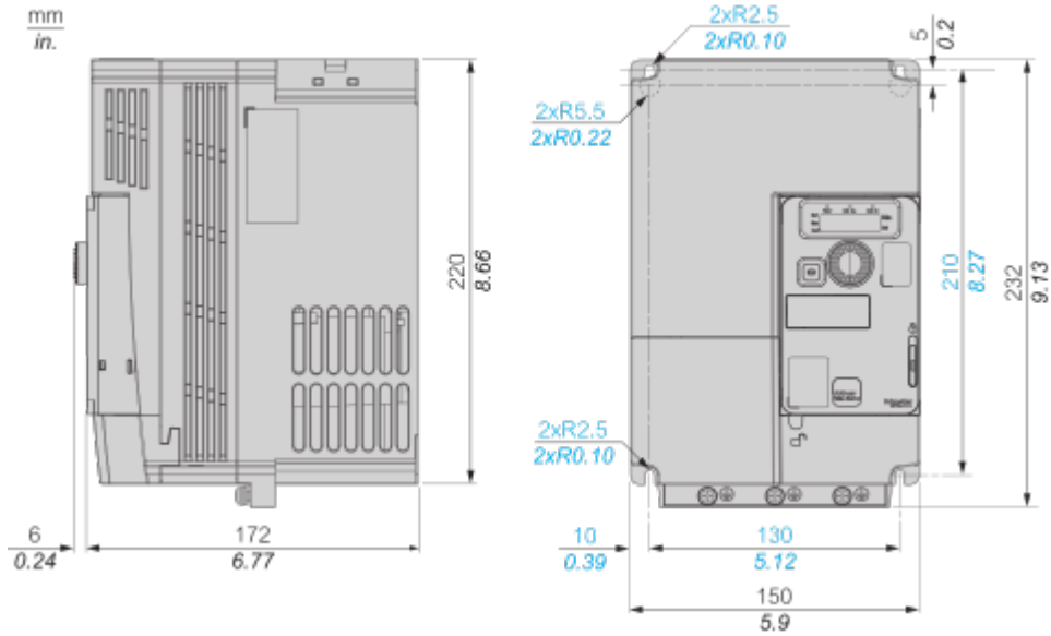
Right and Front View with EMC Plate
