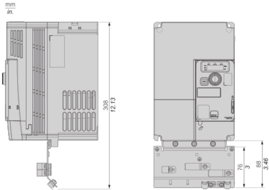
Right and Front View with EMC Plate
