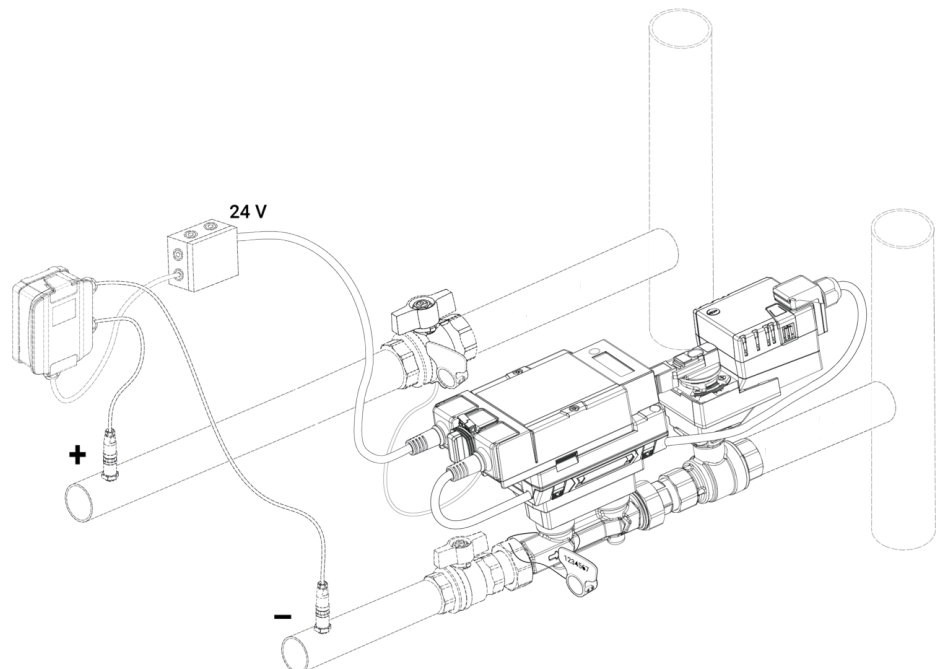
Energy Valve with accessories Differential pressure sensor 22PDP-18.. MID accessory kit EV EXT-EF-..C
