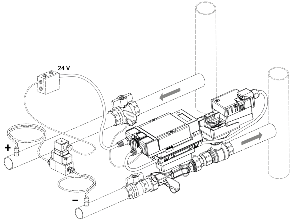
Energy Valve with accessories Differential pressure sensor 22WDP-11.. MID accessory kit EV EXT-EF-..C
