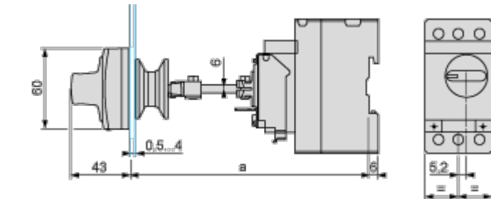
Door cut-out
